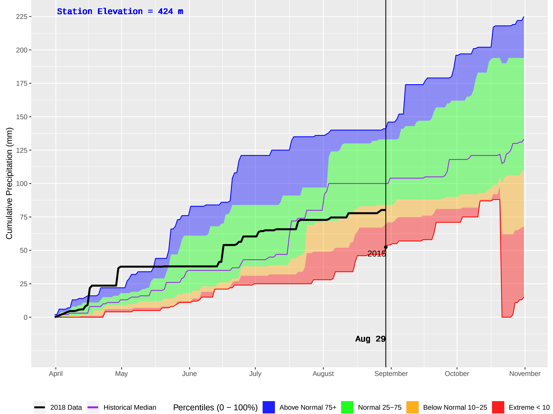
SPLINTLUM (1055) : Historical (2009–2016) and Current (2018) Daily Cumulative Precipitation
