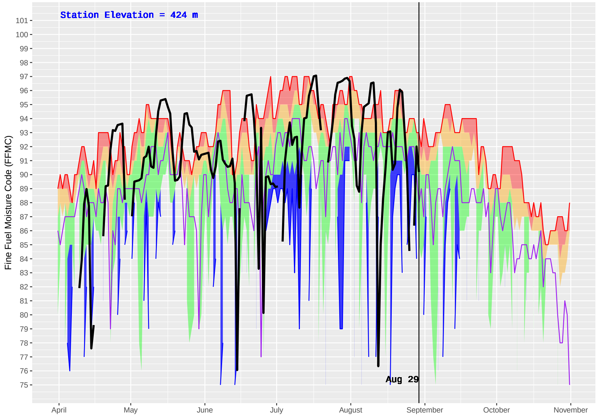
SPLINTLUM (1055) : Historical (2009–2016) and Current (2018) Daily Fine Fuel Moisture Code (FFMC)
