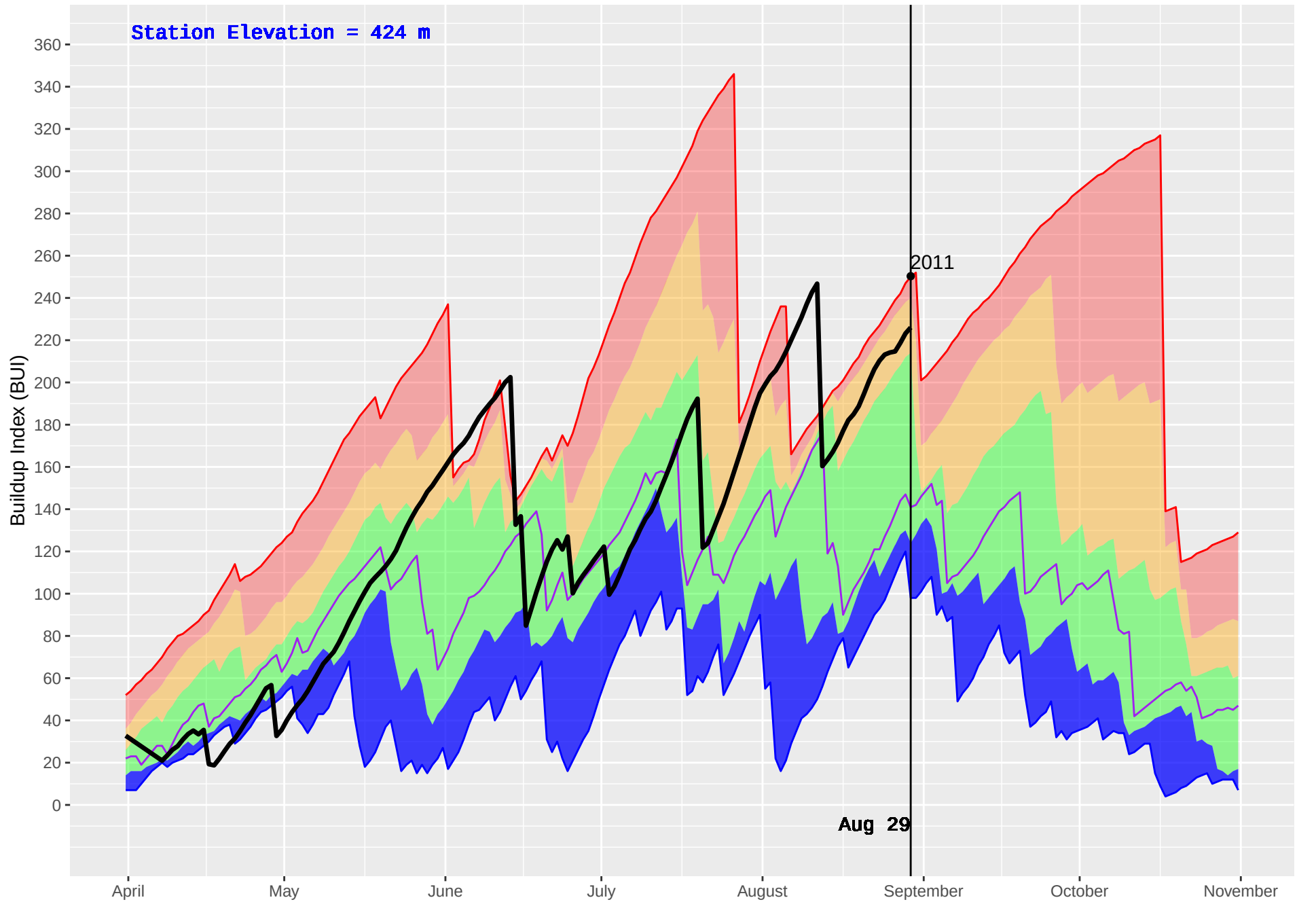
SPLINTLUM (1055) : Historical (2009–2016) and Current (2018) Daily Buildup Index (BUI)
