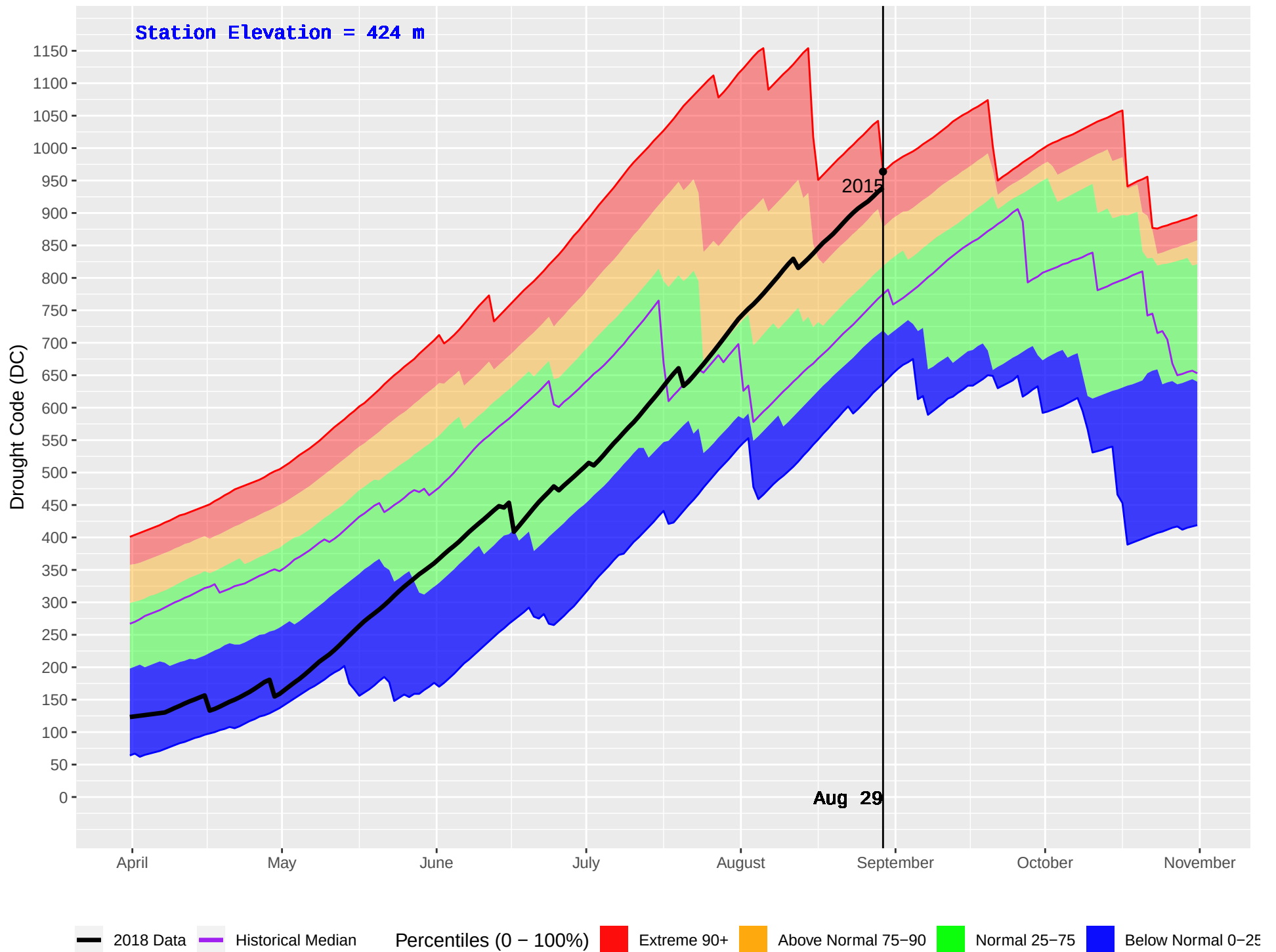
SPLINTLUM (1055) : Historical (2009–2016) and Current (2018) Daily Drought Code (DC)
