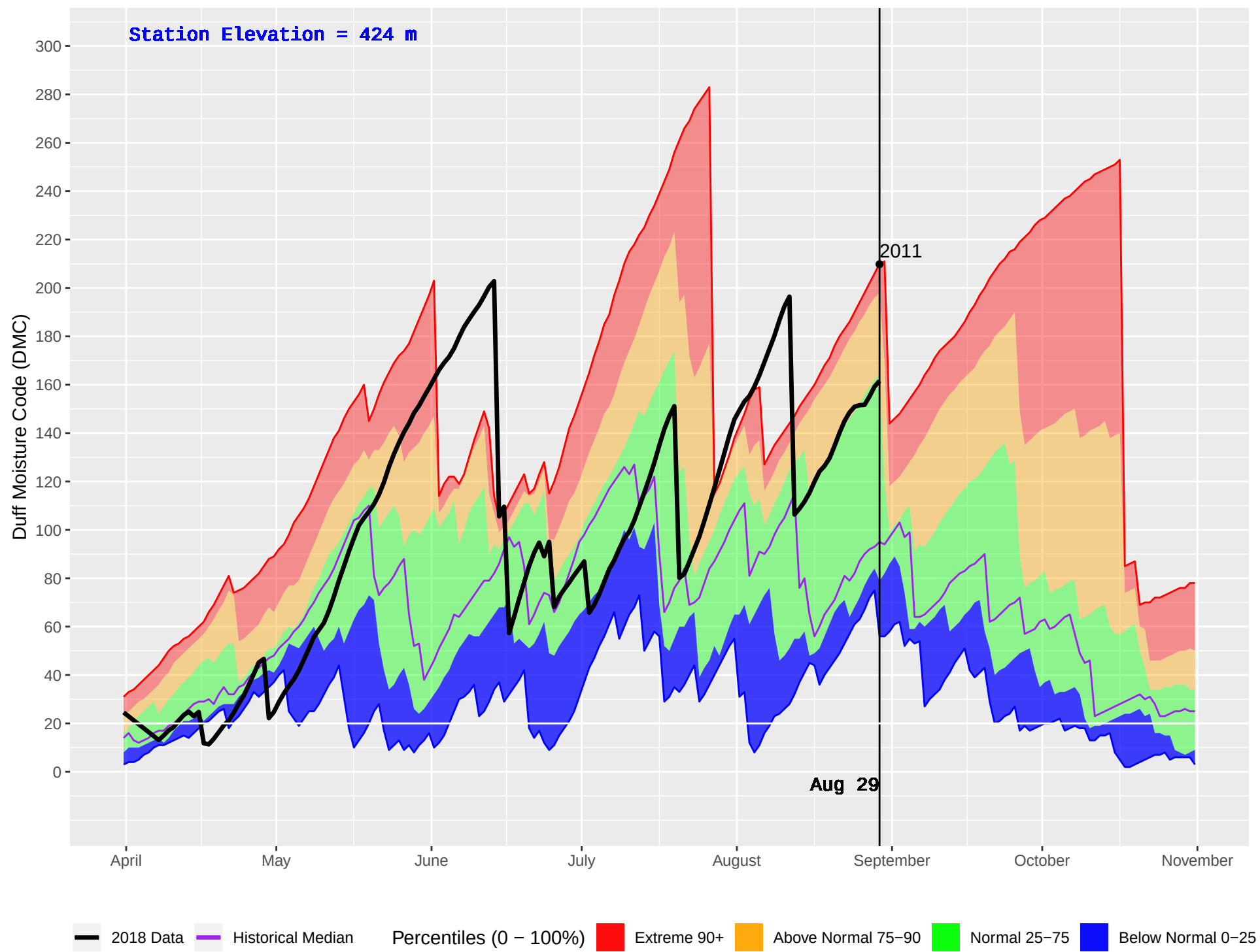
SPLINTLUM (1055) : Historical (2009–2016) and Current (2018) Daily Duff Moisture Code (DMC)
