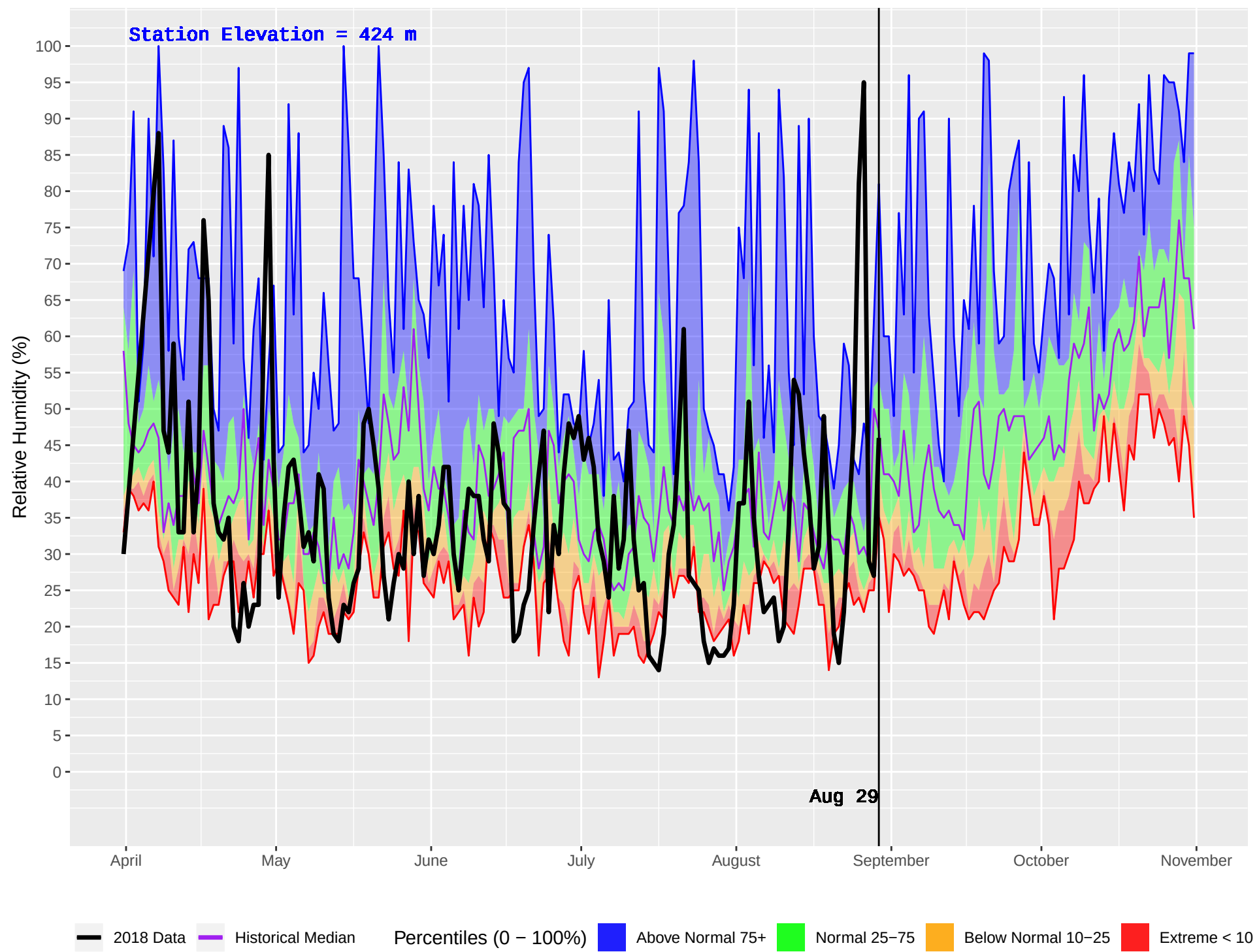
SPLINTLUM (1055) : Historical (2009–2016) and Current (2018) Daily Relative Humidity
